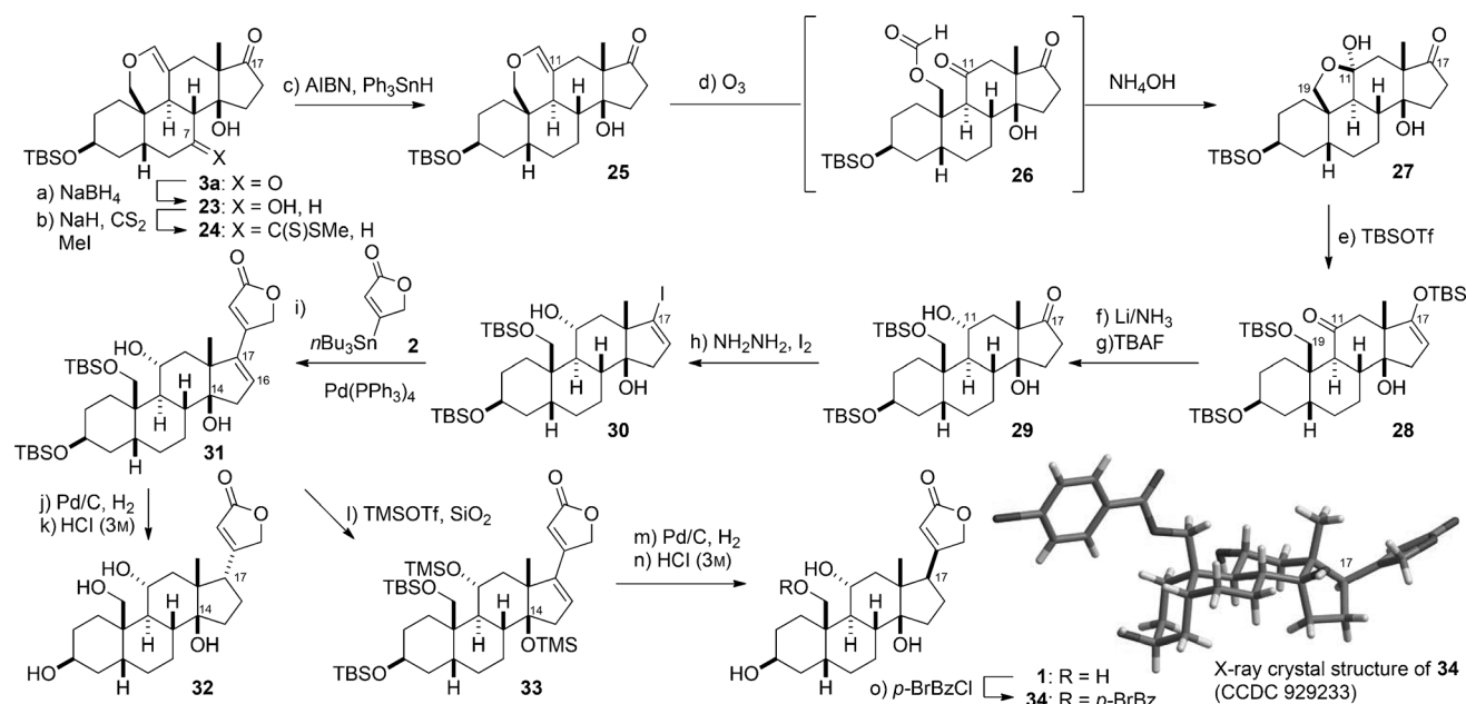
Scheme 4. Reagents and conditions: a) \text{NaBH}_4 , THF, RT, ( 23 \alpha / 23 \beta = 2:1); b) \text{NaH} , THF; \text{CS}_2 , MeI, -50^\circ\text{C} ; c) AIBN, \text{Ph}_3\text{SnH} , benzene, reflux, 50% (3 steps); d) \text{O}_3 , MeOH, -78^\circ\text{C} ; \text{Me}_2\text{S} , RT; \text{NH}_4\text{OH} , 75%; e) TBSOTf, \text{Et}_3\text{N} , \text{CH}_2\text{Cl}_2 , -60^\circ\text{C} ; \text{LiN}(\text{TMS})_2 , RT, 83%; f) \text{Li} , \text{NH}_3 , THF, -78^\circ\text{C} , 95%; g) TBAF, THF, -78^\circ\text{C} , 94%; h) (\text{H}_2\text{N})_2 \cdot \text{H}_2\text{O} , \text{Et}_3\text{N} , EtOH, 50^\circ\text{C} ; \text{I}_2 , \text{Et}_3\text{N} , THF, RT, 91%; i) 2 , \text{Pd}(\text{PPh}_3)_4 (20 mol%), \text{LiCl} , \text{CuCl} , DMSO, 60^\circ\text{C} , 89%; j) \text{Pd/C} , \text{H}_2 , AcOEt, RT; k) \text{HCl} (3 M), MeOH, RT, 78% (2 steps); l) TMSOTf, 2,6-lutidine, \text{CH}_2\text{Cl}_2 , RT; \text{SiO}_2 , 73%; m) \text{Pd/C} , \text{H}_2 , AcOEt, RT, 73%; n) \text{HCl} (3 M), MeOH, RT, 82%; o) p -BrBzCl, DMAP, \text{CH}_2\text{Cl}_2 , RT, 65%. AIBN = 2,2'-azobisisobutyronitrile, Bz = benzoyl, DMSO = dimethylsulfoxide.
